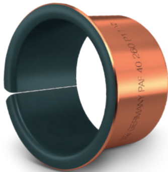
KS PERMAGLIDE® Bundbuchse Bauart PAF ... P11
